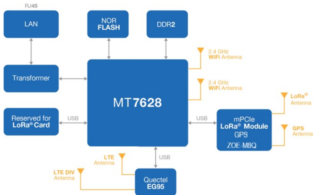
Figure 2: RAK7289CV2 WisGate Edge Pro V2 with LTE block diagram
