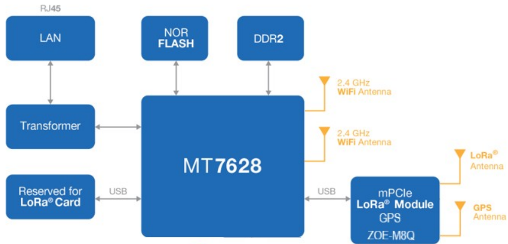
Figure 1: RAK7289V2 WisGate Edge Pro V2 without LTE block diagram
