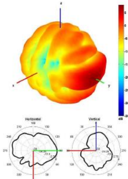
6500 MHz Radiation pattern
