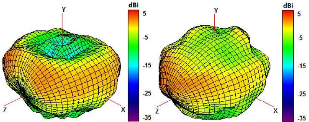
2100 and 2600 MHz Radiation pattern
