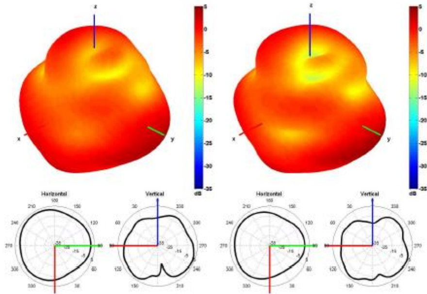
868 and 915 MHz Radiation pattern
