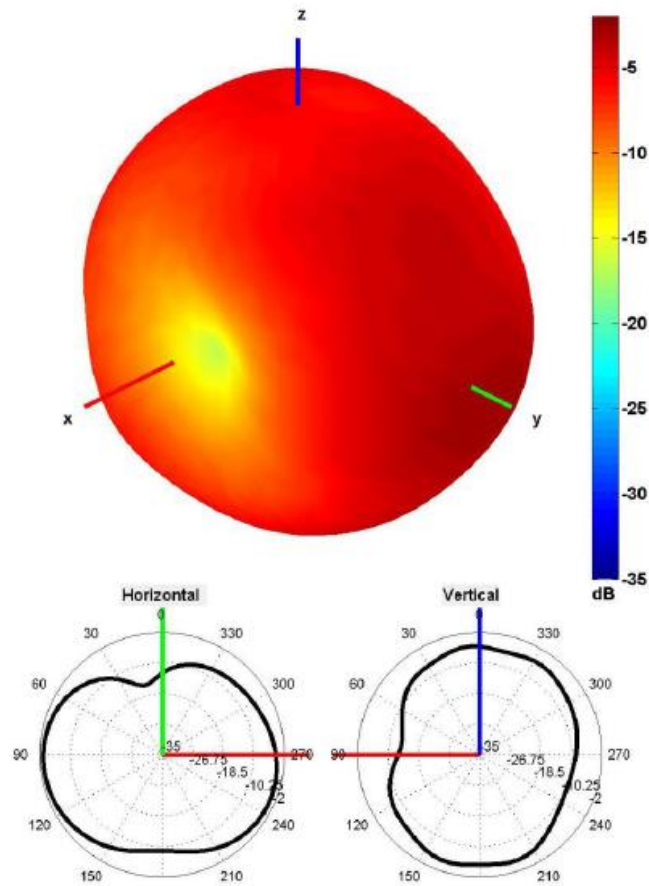
433 MHz Radiation pattern
