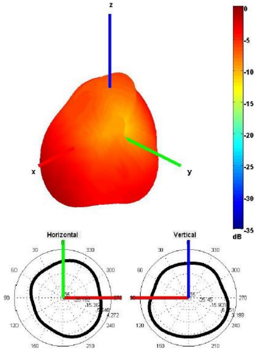
915 MHz Radiation pattern
