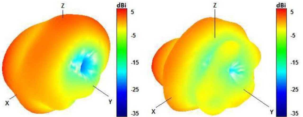
2100 and 2600 MHz Radiation pattern
