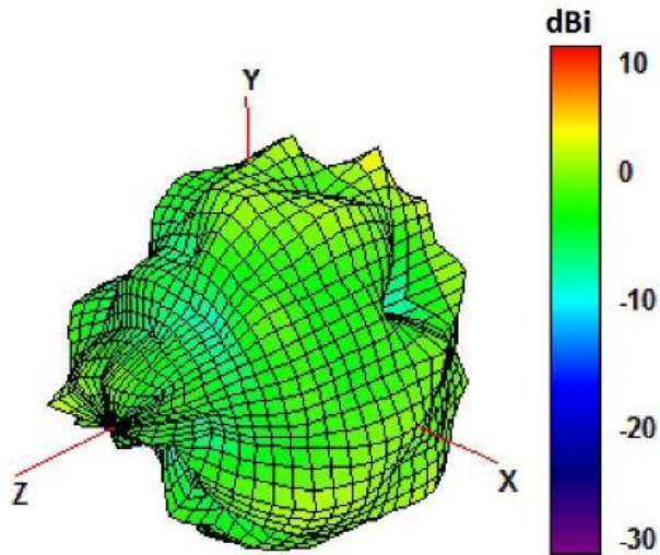
6500 MHz Radiation pattern
